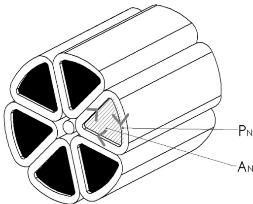
Figure 2: Axial motor winding
