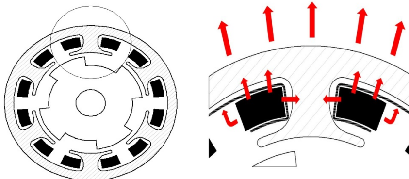
Figure 7: Radial Motor Thermal Path
