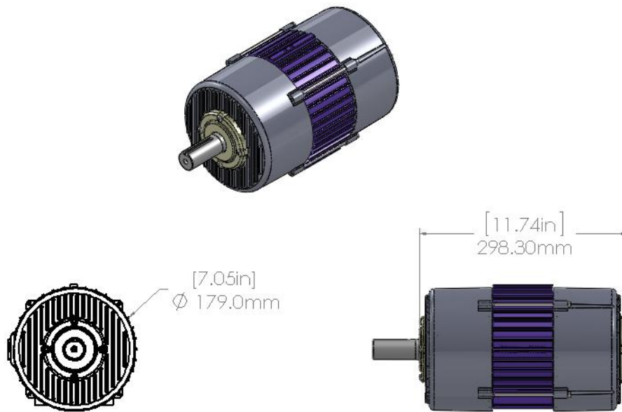
Figure 9: Axial Permanent Magnet 3.7 Kw Motor
