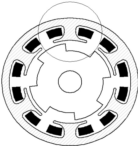
Figure 1A: Radial motor winding
