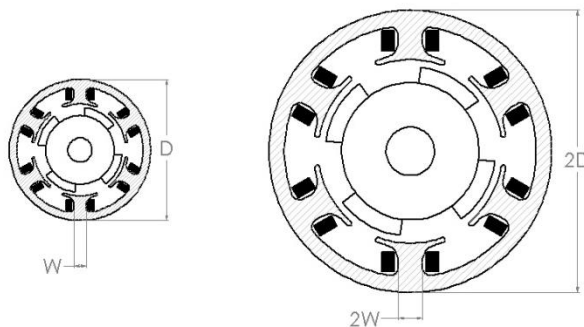
Figure 5: Radial motor with diameter D and 2D
