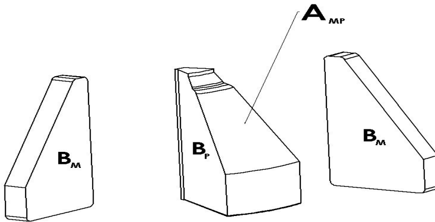
Figure 3: IPM spoke type flux concentration
